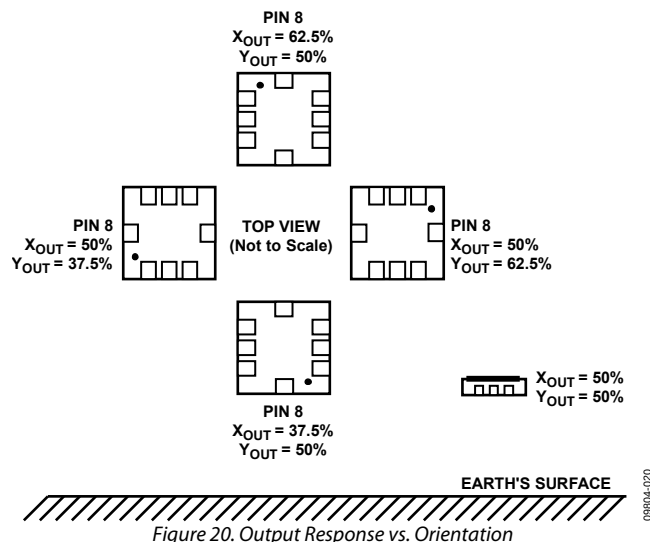
Figure 20. Output Response vs. Orientation
